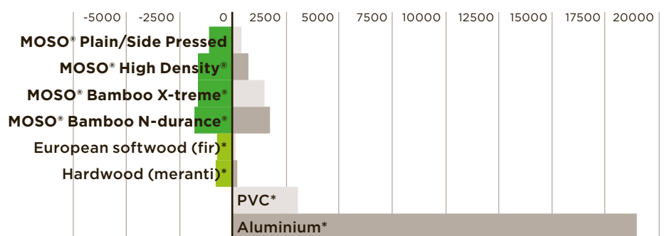
CO 2 storage vs. CO 2 emissions during production and transport
