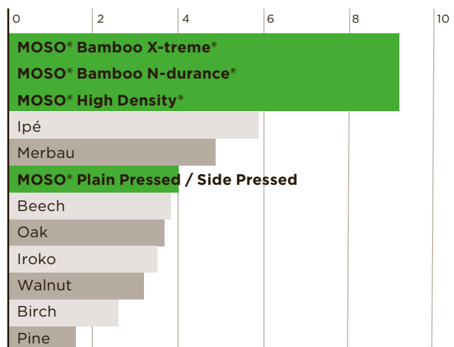
Average brinell hardness
