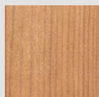
HOTwood pine
